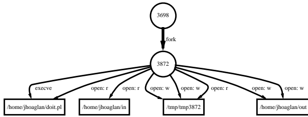
Figure 5b. FAB presentation of “Finding a File’s Origin” situation with the focus on the process 3872. It is shown that “/home/jhoaglan/doi.pl” is “exec”ed by that process and a couple files besides “/tmp/tmp3872” are read from and written to.
