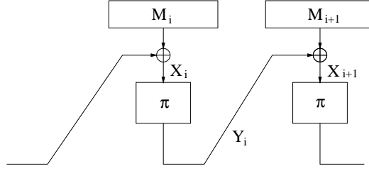
Fig. 6. The labeling convention used in the proof of Lemma 3.
