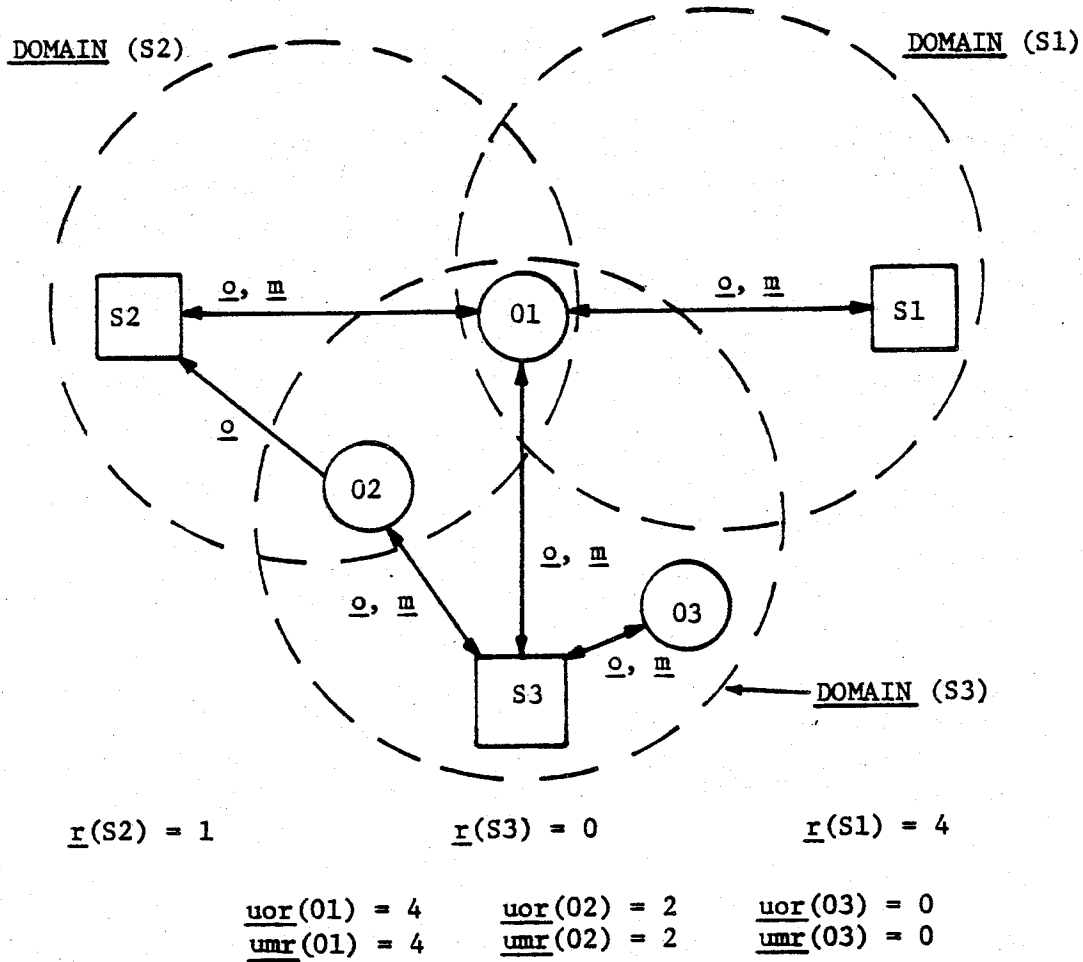
Figure 9. Rings
