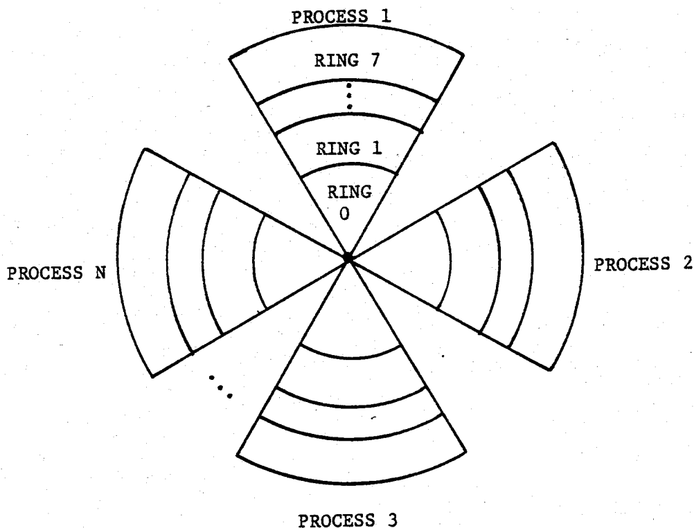
Figure 10. Subject/Process Structure
