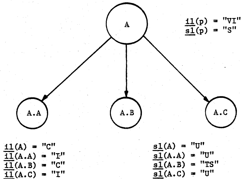
Figure 12. Inaccessible Objects
