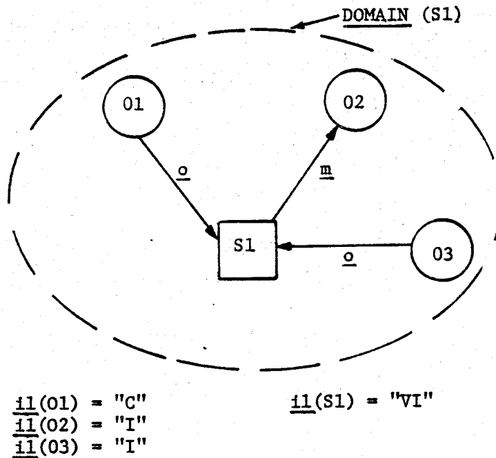
Figure 6. Ring Policy
