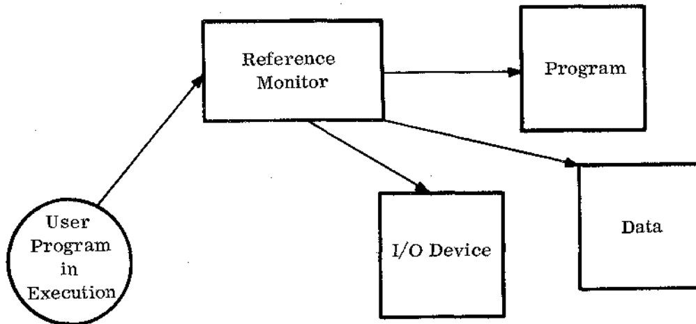
Figure 1. Reference Monitor
